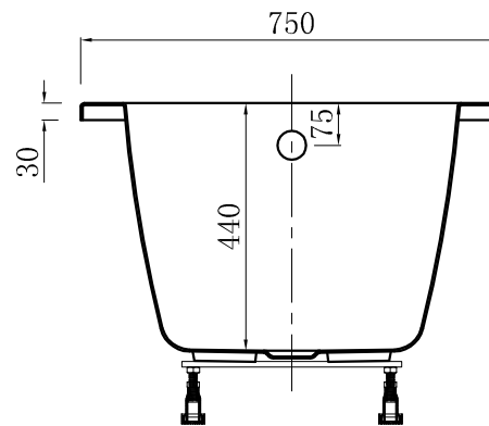
Section F-F
